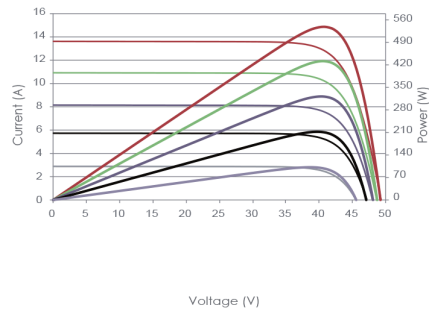
Current-Voltage & Power-Voltage Curves (540W)
