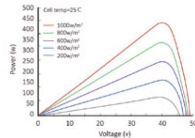
Power-Voltage Curve (LR4-72HPH-440M)
